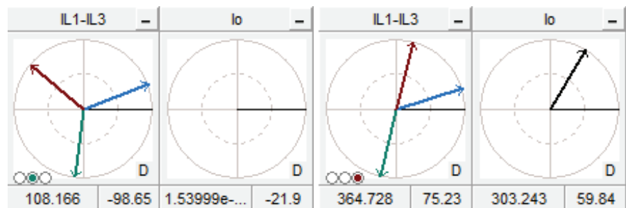
Figure 5.19: Phase L3 forward
