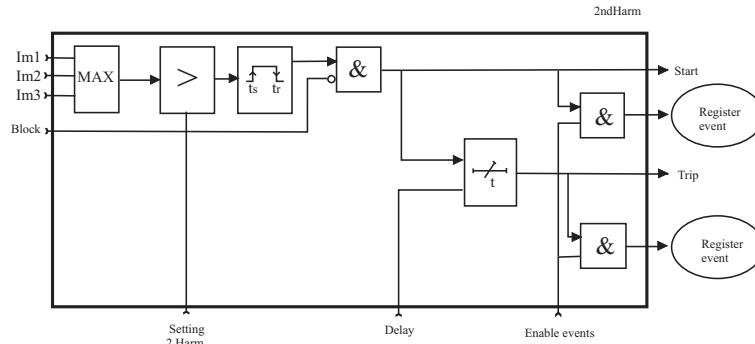
Figure 5.22: Block diagram of the magnetising inrush stage.
