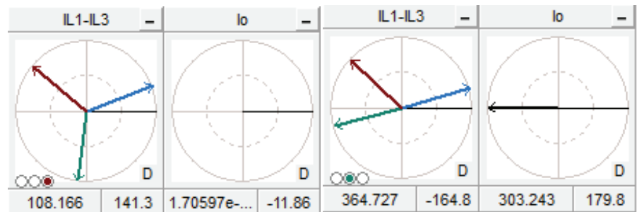
Figure 5.18: Phase L2 forward
