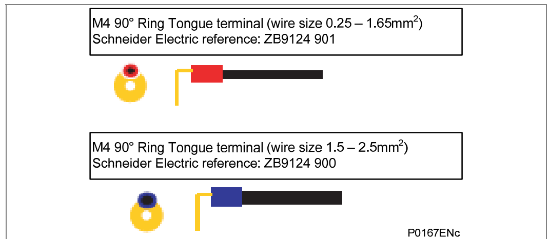
Figure 2 - Connection of Ring Tongue Terminals
