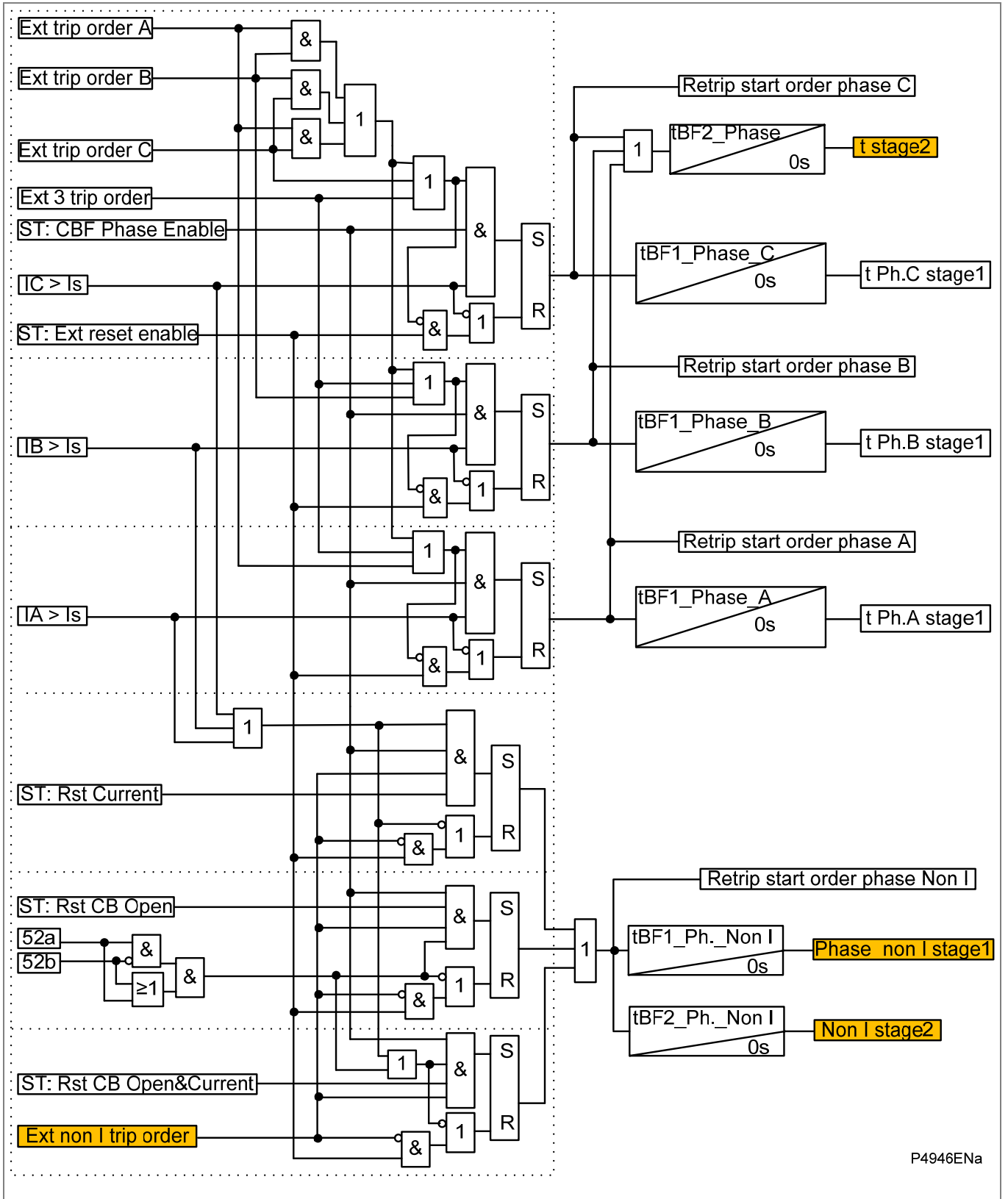
Figure 3 - Phase element logic
