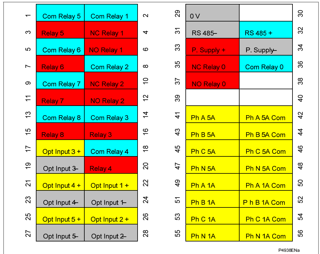
Figure 4 - Rear connectors
