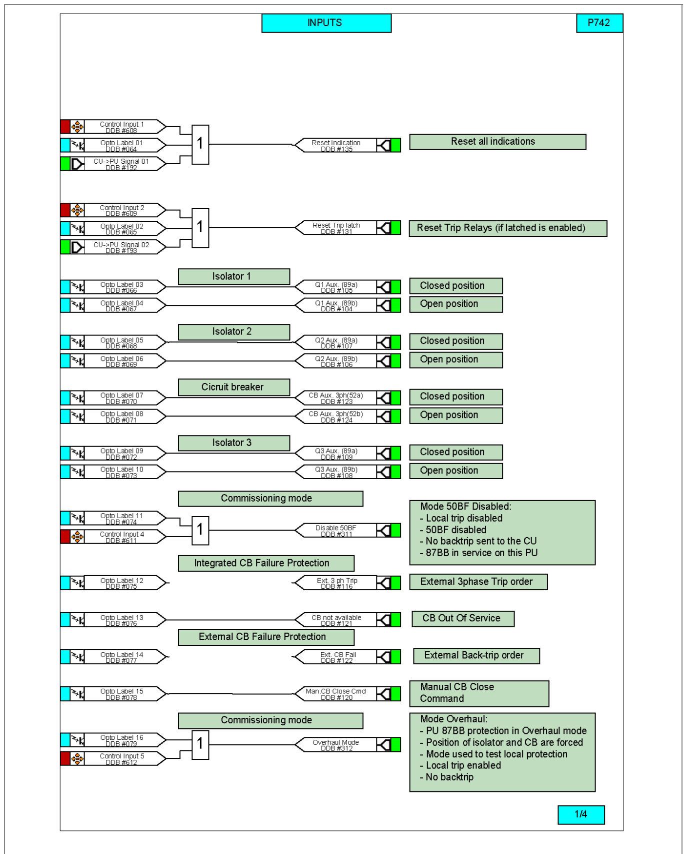
Figure 5 - P742 PSL Diagram 1 of 4
