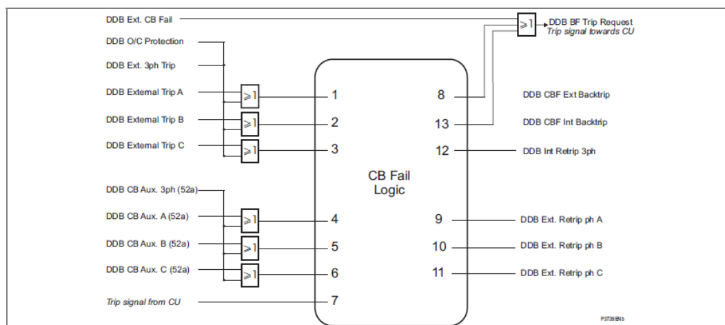
Figure 9 - CB fail logic (DDB inputs &amp; outputs)
