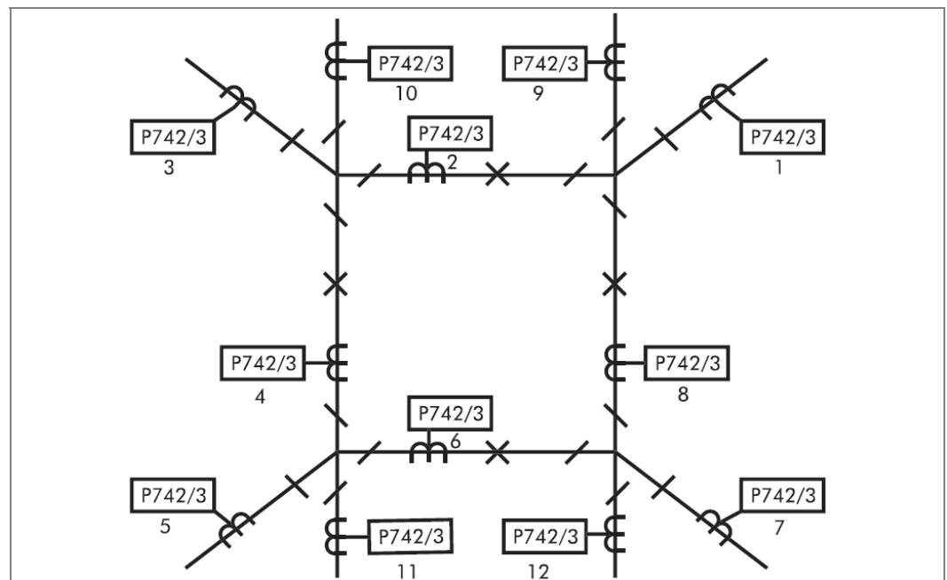
Figure 39 - Mesh corner
