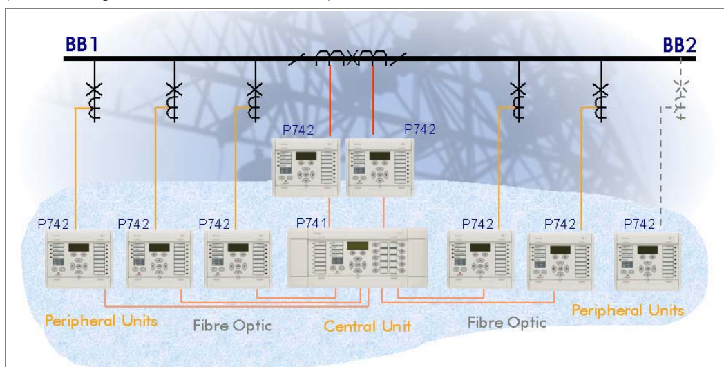
Figure 29 - Module interconnection
