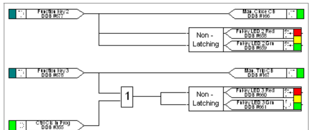
Figure 32 - CB control via function keys default PSL
