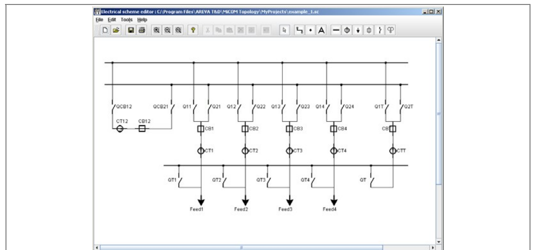
Figure 10 - P740 Scheme Editor
