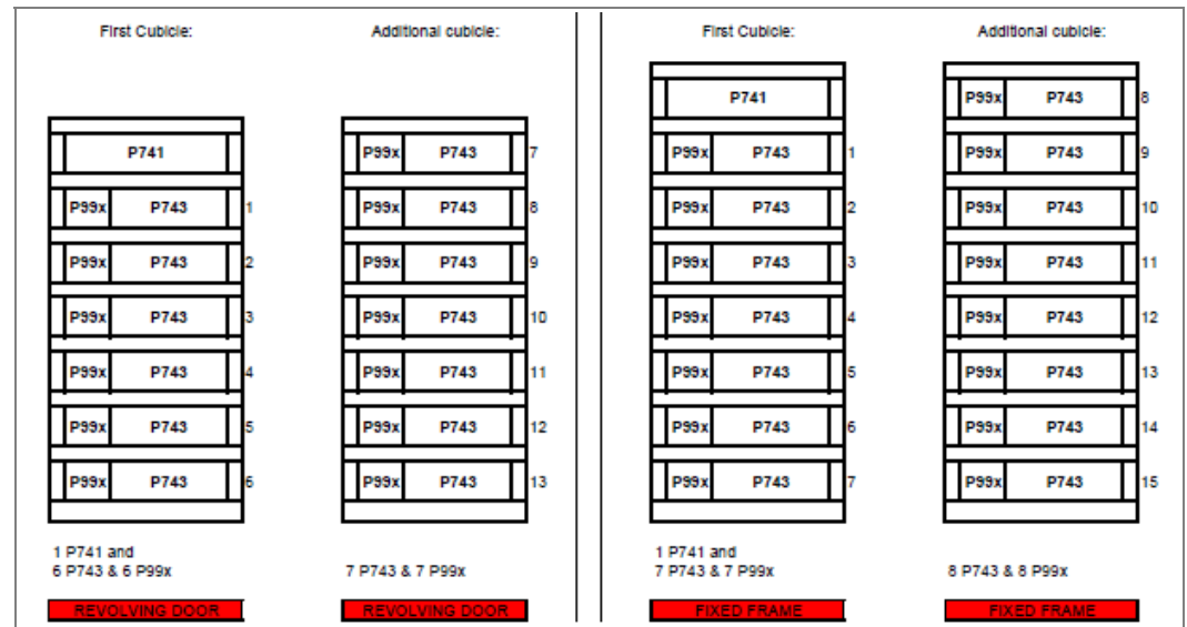
Figure 27 - 1 P741 and P743 with (or without) P99X test block
