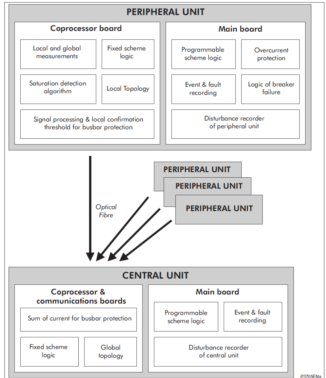
Figure 11 - System overview
