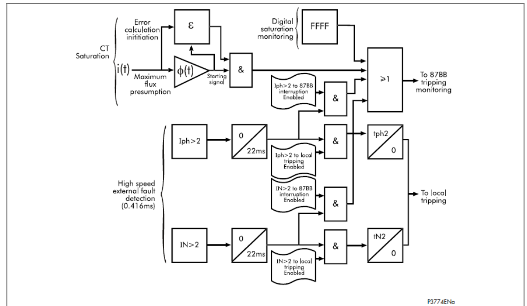
Figure 25 - Determination of signal quality in the peripheral unit
