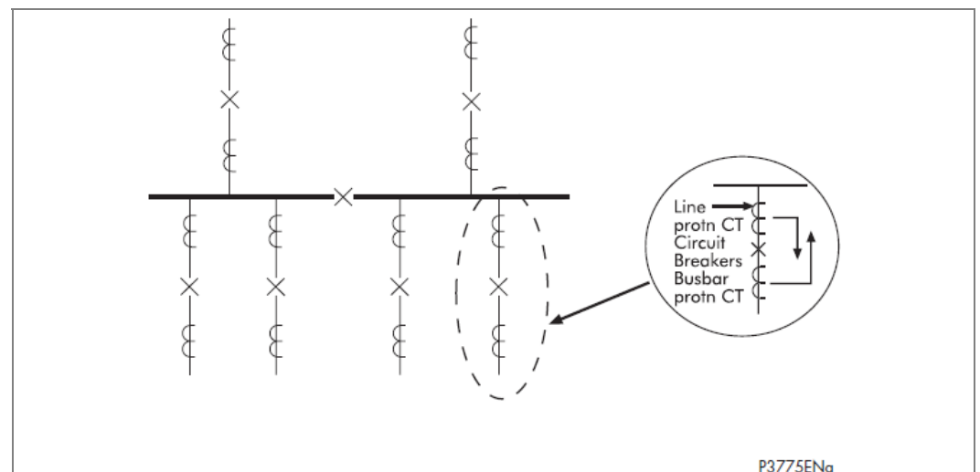
Figure 26 - CT location
